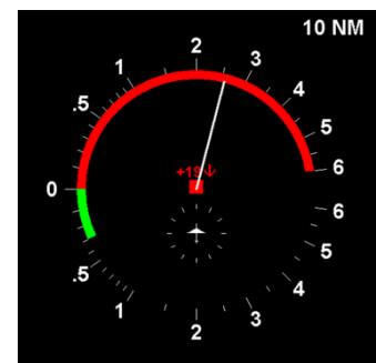
Figure 3: Initial Level Off RA as shown on a generic IVSI display (incorporating a traffic display).
